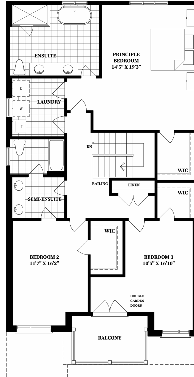
Second Floor - Elev A Alternative (3 Bed)
